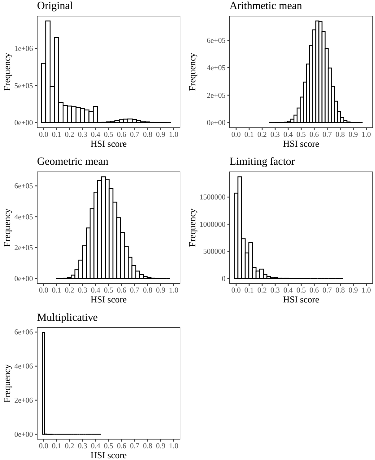
Figure 2. Empirical distributions of HSI scores for the creekhubRivLargerStrmDistWithin5km model using the original author-specified model equation from McMahon (1982), and an arithmetic mean, geometric mean, limiting factor, and multiplicative structure incorporating all SIV variables. Note differences in the y axis.
