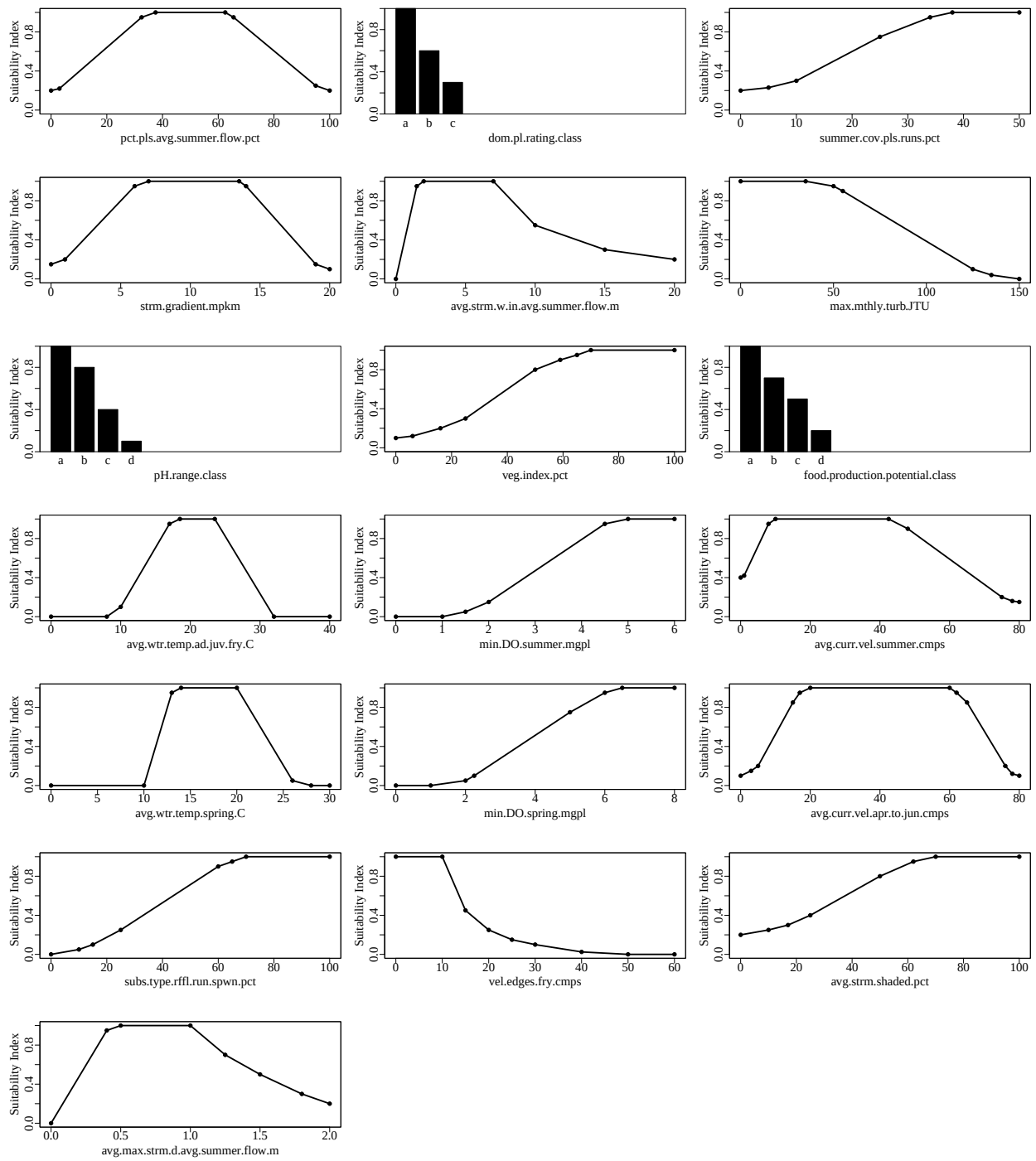
Figure 1. Suitability index graphs for variables included in the creekchubRivLargerStrmDistWithin5km model in ecoest.
